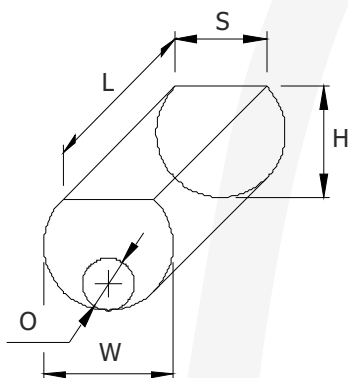
"OS" (Omega Section)
